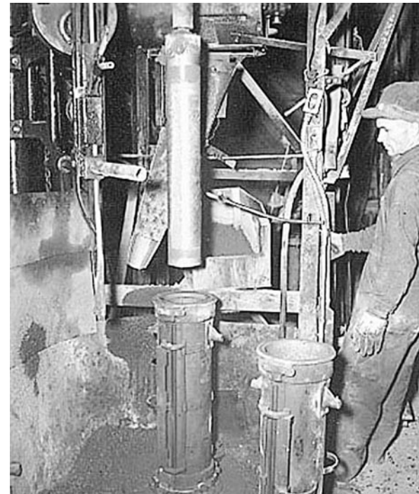
Early production of small diameter concrete drainage tile using a mechanized process. Photo: Courtesy of American Concrete Pipe Association
